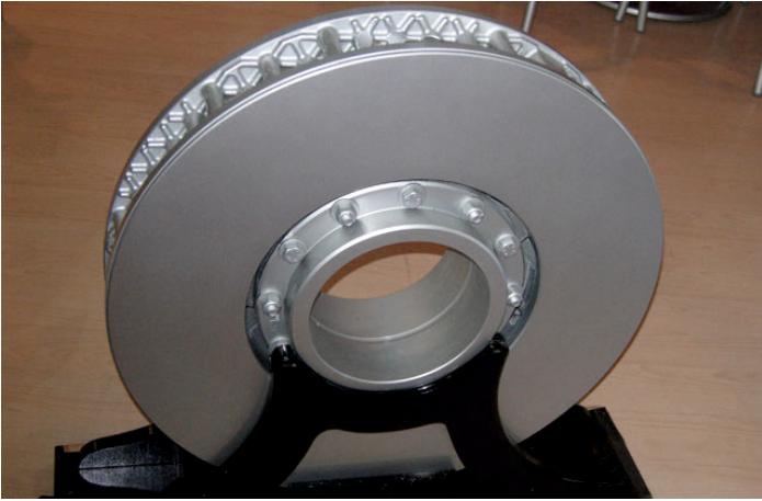
FREN DİSKİ
